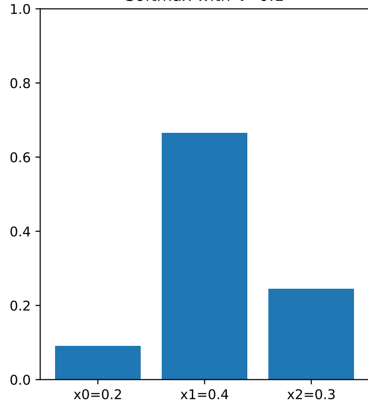
Softmax with \tau=0.1
